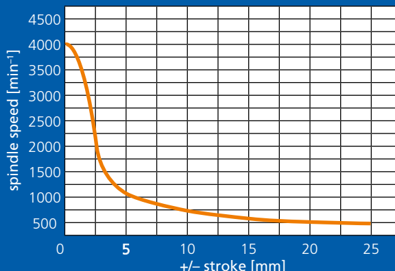
Max. stroke/spindle speed diagram
